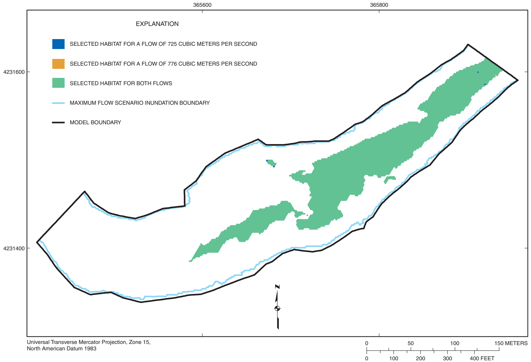
Figure 4-47. Selected habitat area distribution for habitat category 7 (paddlefish) at flows of 725 and 776 cubic meters per second at Marais des Cygnes River site MDC2.
